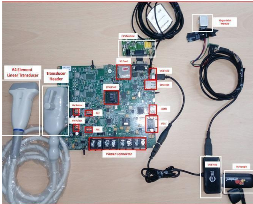
IOT Enabled Ultrasound System Based on ZYNQ processor
