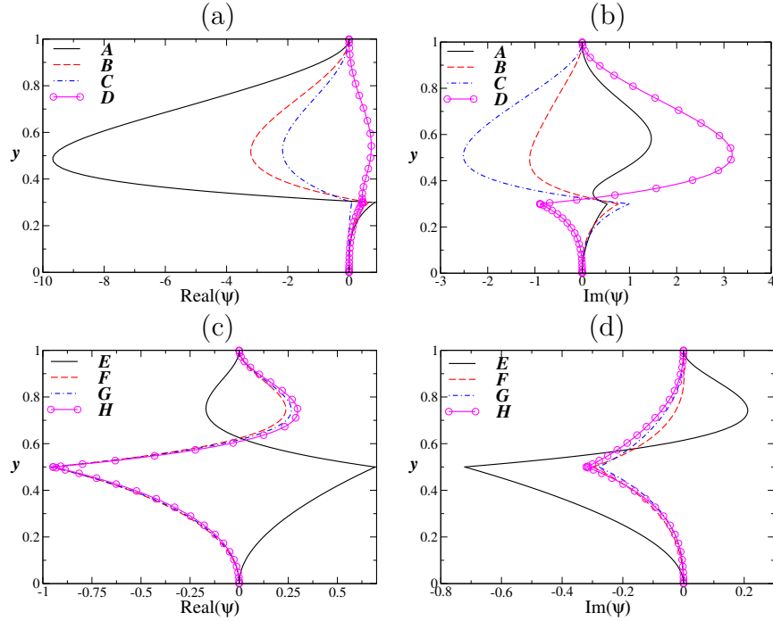
Figure 5: The real and imaginary parts of the streamfunction eigenfunctions ( \psi_1, \psi_2 ). (a,b) for points A, B, C and D in Fig. 4(a) ( h^0 = 0.3 ) and (c,d) for points E, F, G and H in Fig. 4(b) ( h^0 = 0.5 ).
