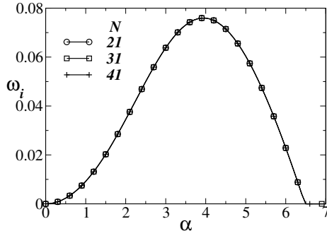
Figure 3: The effect of increasing the order of Chebyshev polynomials, N , on the variation of \omega_i with \alpha (dispersion curve) obtained using a typical set of parameters, i.e Re = 10 , m = 10 , n = 1 , \Gamma = 1 , h^0 = 0.3 , \epsilon_r = 2 , \sigma_r = 10 , E_0 = 1 and Bn = 5 .
