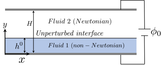
Figure 1: The schematic diagram of the flow configuration considered. Fluid 1 is a non-Newtonian fluid characterised by a Herschel-Bulkley model, whereas Fluid 2 is a Newtonian fluid. The height of the channel is H and the fluids are separated by a sharp interface at y = h^0 . The wall at y = 0 is grounded and an electric field of potential \phi_0 is applied between the walls in y direction.
