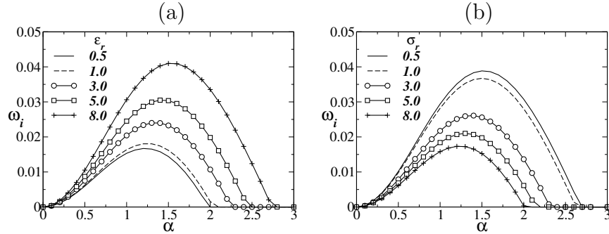
Figure 6: The effect of (a) the electric permittivity ratio, \epsilon_r for \sigma_r = 5.0 and (b) the electrical conductivity ratio, \sigma_r for \epsilon_r = 2.0 on the dispersion curves. The rest of the parameters used are h^0 = 0.5 , Bn = 5 , E_0 = 1 , Re = 10 , m = 10 and \Gamma = 1 .
