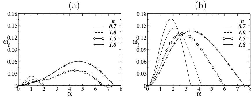
Figure 9: The effect of flow index, n on the dispersion curves ( \omega_i versus \alpha ) for (a) E_0 = 0 (without electric field) and (b) E_0 = 2.0 . Here, h^0 = 0.5 , Bn = 2 and rest of the parameters are the same as the “base parameters”.
