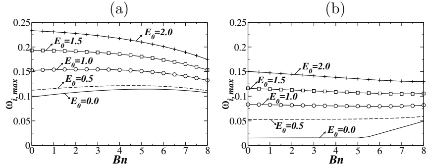
Figure 8: Effect of the Bingham number, Bn on the growth rate of the most dangerous mode, \omega_{i,max} for different values of the electric Weber number E_0 . (a) h^0 = 0.3 and (b) h^0 = 0.5 . Here, n = 1 and the rest of the parameters are the same as the “base parameters”.
