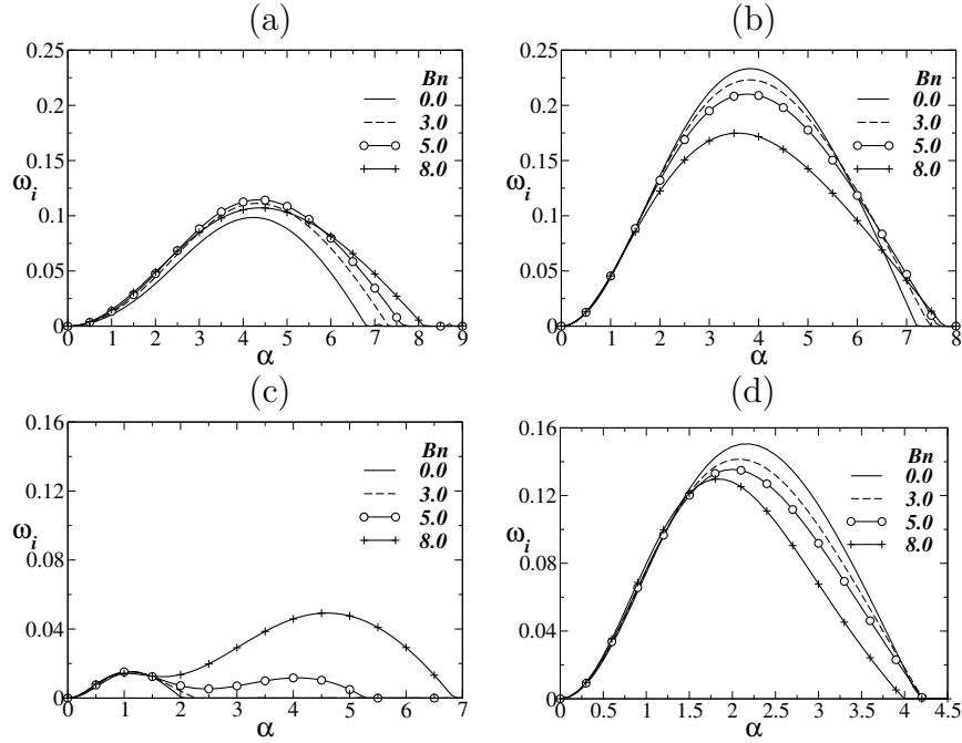
Figure 7: Effect of the Bingham number, Bn on the dispersion curves ( \omega_i versus \alpha ) for (a,c) E_0 = 0 (without electric field) and (b,d) E_0 = 2.0 . Here, panels (a,b) and (c,d) are for h^0 = 0.3 and h^0 = 0.5 , respectively. Here, n = 1 and the rest of the parameters are the same as the “base parameters”.
