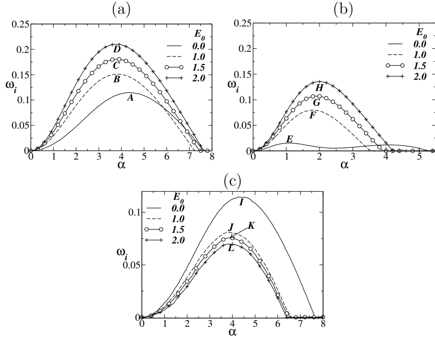
Figure 4: Effect of the electric Weber number, E_0 , on the dispersion curve ( \omega_i versus \alpha ) for Bn = 5 and n = 1 . (a) h = 0.3 and (b) h = 0.5 for \epsilon_r = 10 and \sigma_r = 2 ; (c) h = 0.3 for \epsilon_r = 2 and \sigma_r = 5 . The rest of the parameters considered are Re = 10 , m = 10 and \Gamma = 1 .
