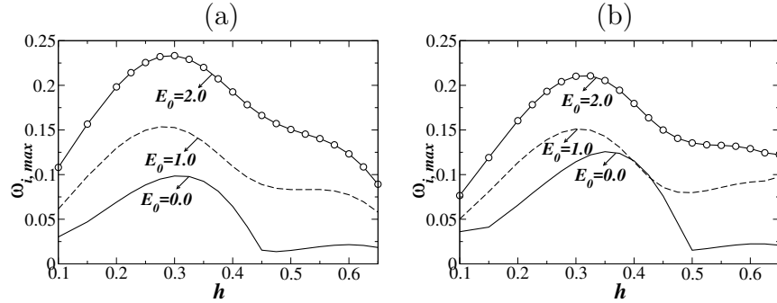
Figure 10: Effect of the thickness of the bottom layer, h^0 on the growth rate of the most unstable mode, \omega_{i,max} for different values of E_0 . (a) Bn = 0 (Newtonian layer) and (b) Bn = 5 (Bingham fluid layer). Here, n = 1 and the rest of the parameters are the same as the “base parameters”.
