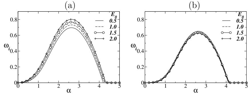
Figure 11: Effect of the electric Weber number, E_0 on the dispersion curve ( \omega_i versus \alpha ). (a) \epsilon_r = 10 , \sigma_r = 2 and (b) \epsilon_r = 2 , \sigma_r = 10 . Here, m = 1 (i.e. both fluids having same viscosity) and the rest of the parameters are for Bn = 5 , n = 1 , h = 0.3 , Re = 10 and \Gamma = 1 .
