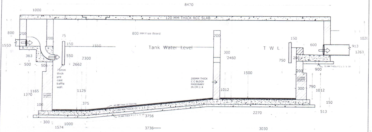
Sectional Elevation
