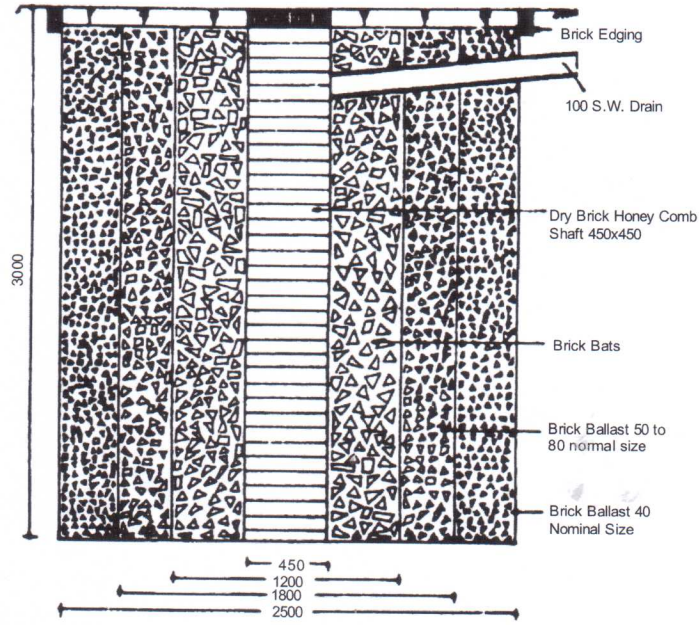
SECTION AB
