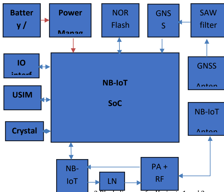
Figure 2 Block diagram for Variants 1 and 2
