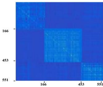
Figure 7: Mean interval kernel representation for motion boundary histogram (MBH) features and uGMM 256 components and 3-class grading score (best viewed in color).
