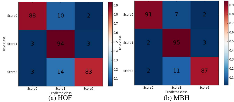
Figure 6: Confusion matrix of HOF and MBH feature vector using GMM-IMK dynamic kernel with SVM for 256 components for 3-class grading scores (best viewed in color).
