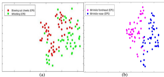
Figure 8: t-sne plot for the expressions of facial paralysis using MBH and GMM-MIK dynamic kernel based SVM for 256 components for 3-class grading score (best viewed in color). In (a) t-sne plot for expression blowing out cheeks (EP6) and whistling (EP8) and in (b) for expression wrinkle forehead (EP1) and wrinkle nose (EP5)
