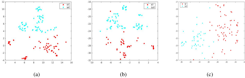
Figure 4: t-SNE plot of attribute vectors for (a) knot tying (KT) vs needle passing (NP) (b) knot tying (KT) vs suturing (SUT) (c) needle passing (NP) vs suturing (SUT) . Here, the axes represent first and second dimensions in the factor analysis
